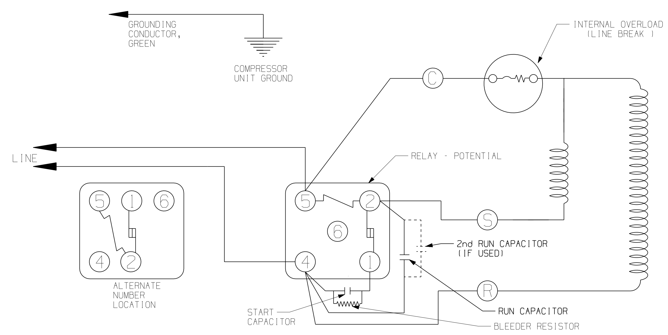
230 VOLT SCHEMATIC WIRING DIAGRAM-CSR OR CSR START CAPACITOR ASSIST - INTERNAL OVERLOAD (LINE BREAK) - REF. DWG. MD472-69
