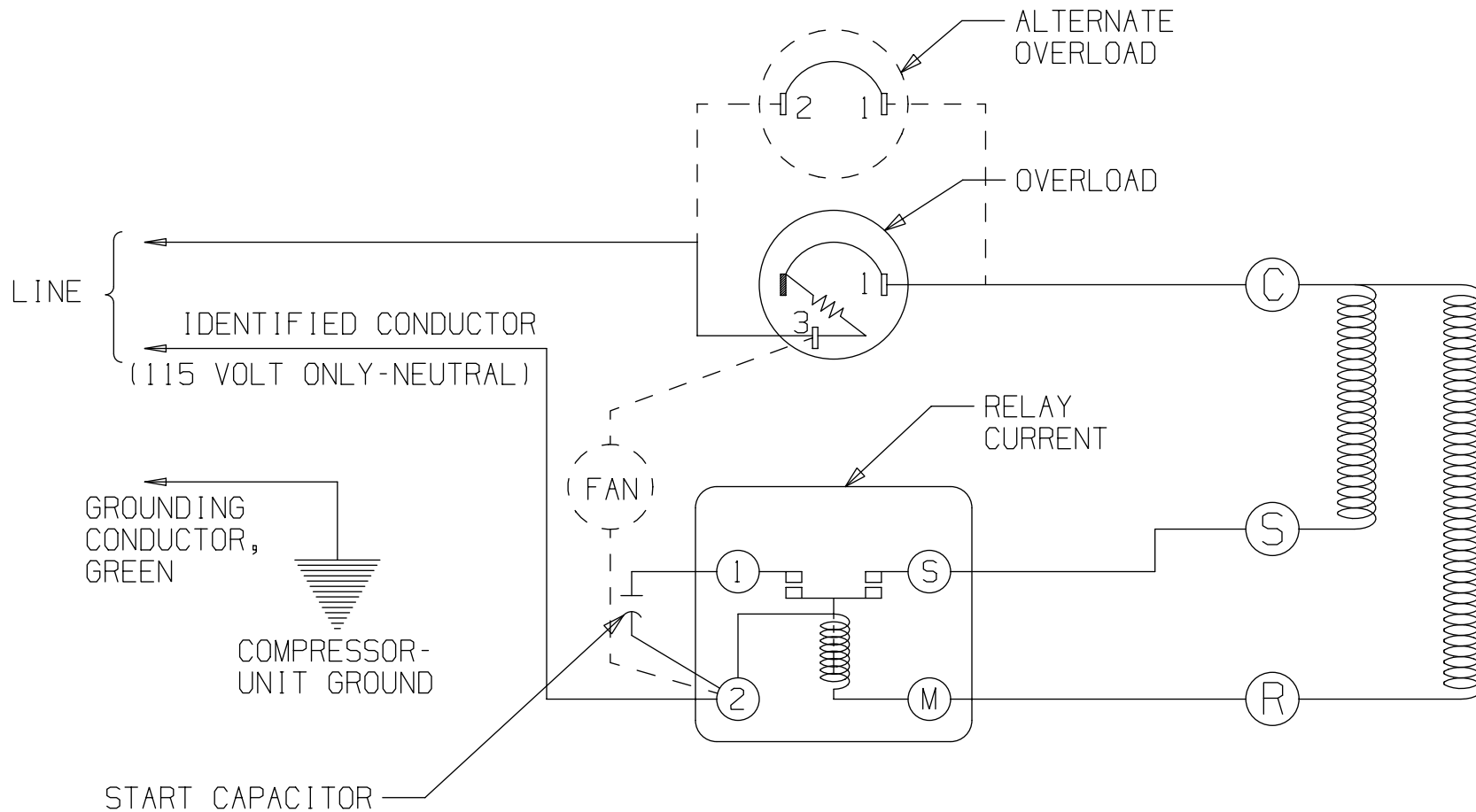
115 OR 230 V SCHEMATIC WIRING DIAGRAM - CSIR
