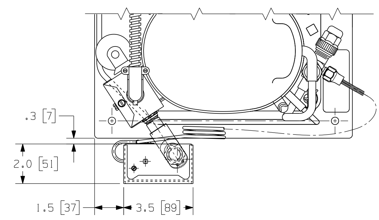
ALTERNATE VIEWS SHOWING PRESSURE SWITCH
