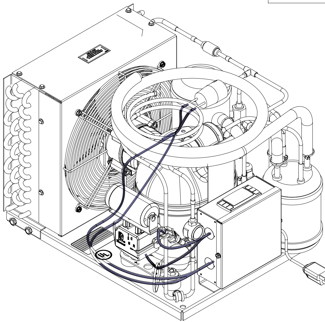
ISOMETRIC VIEW SCALE 4:1
