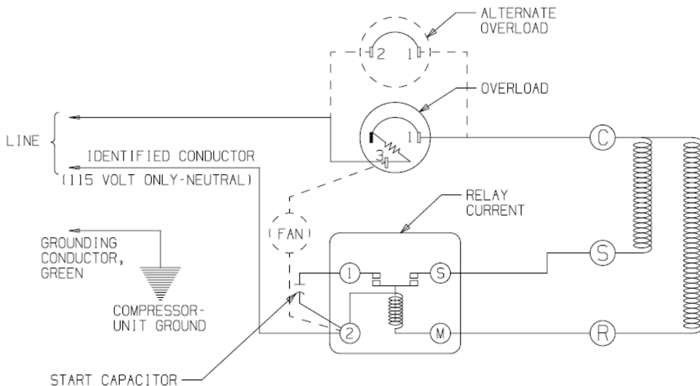
115 OR 230 V SCHEMATIC WIRING DIAGRAM - CS1R
