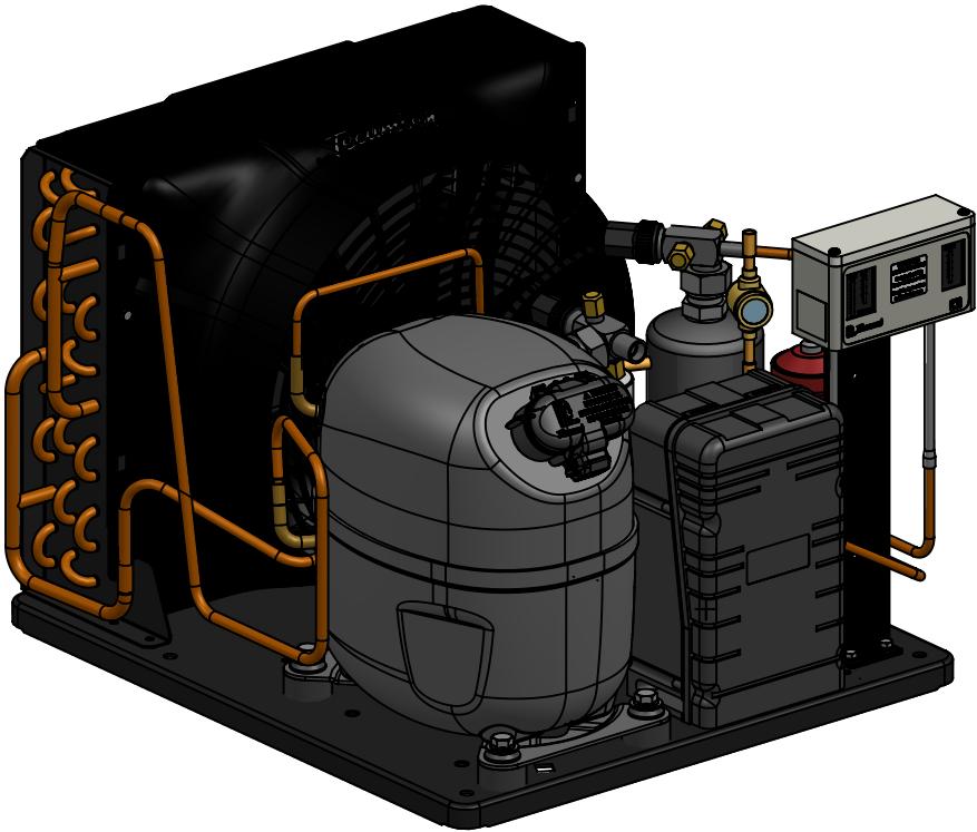
DG7317 Pressostat HP/BP réglable HP/LP adjustable pressure switch
