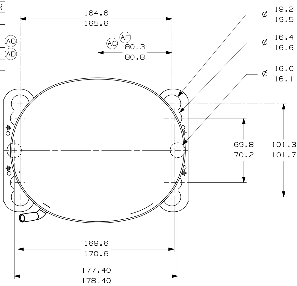
- AUXILIARY VIEW - FASTENING DIMENSIONS
