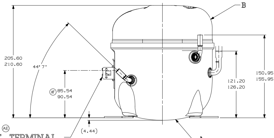
HERMETIC TERMINAL 14945645 WITH SPADE TERMINALS
