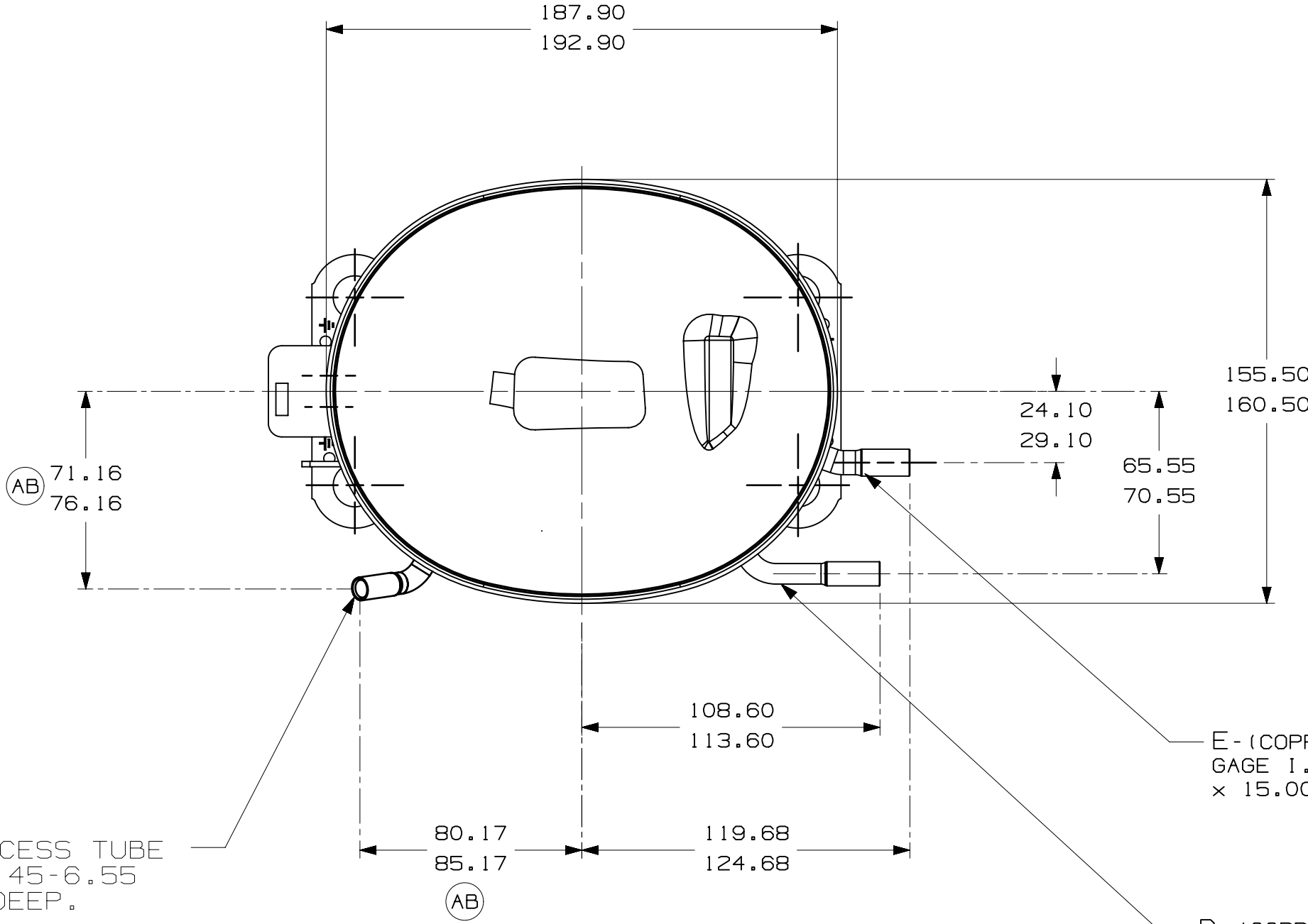
D - (COPPER) DISCHARGE TUBE GAGE I.D. TO 6.45-6.55 × 15.00-17.00 DEEP.
