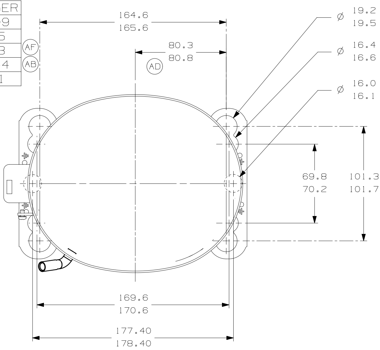
- AUXILIARY VIEW - FASTENING DIMENSIONS
