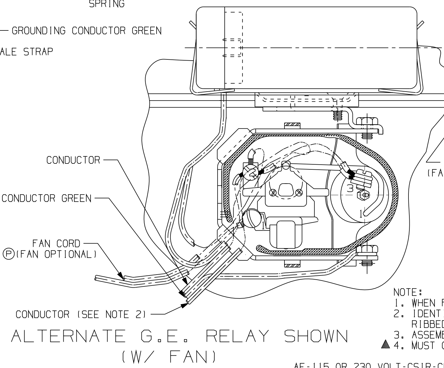
ALTERNATE G.E. RELAY SHOWN (W/ FAN)
