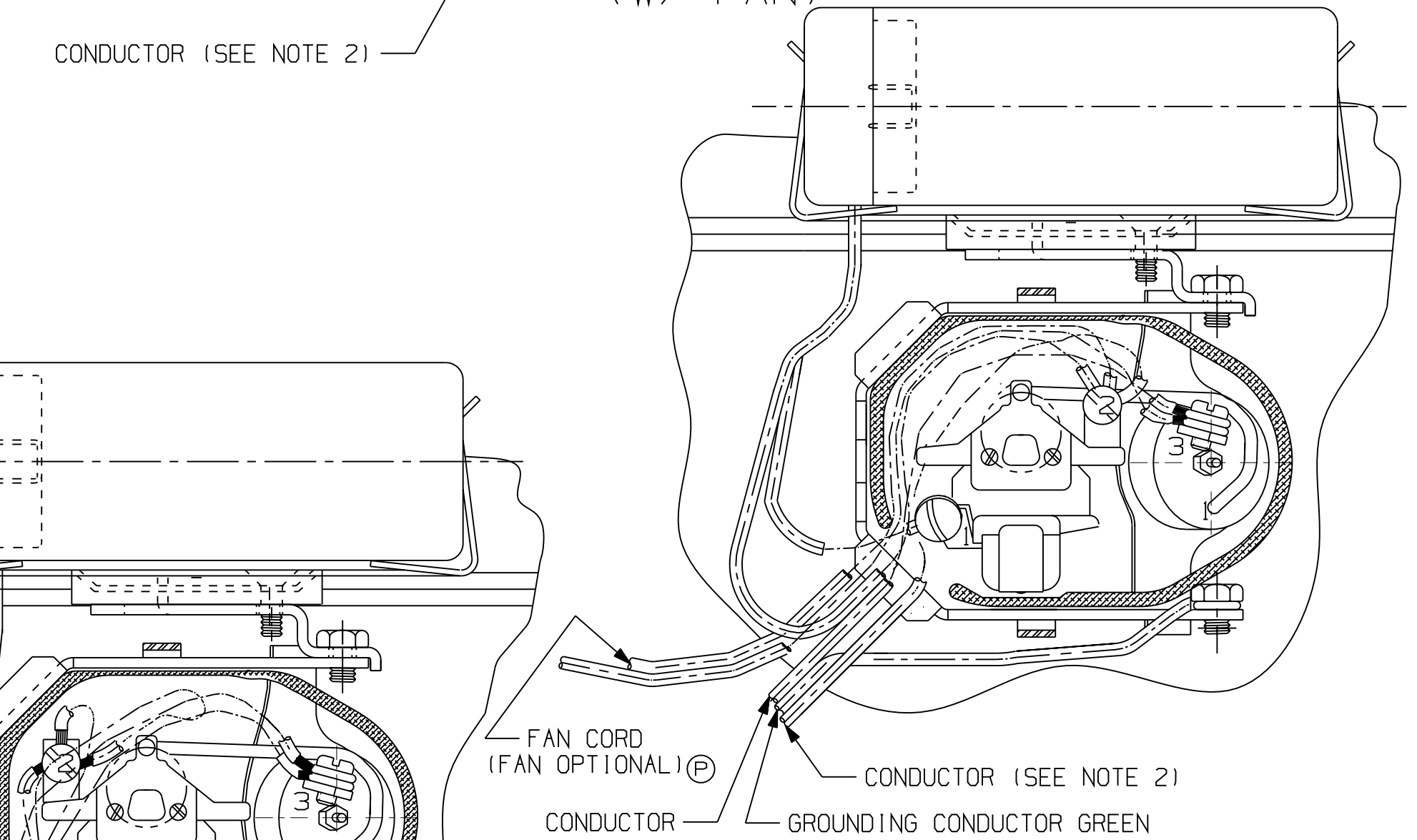
ALTERNATE G.E. RELAY SHOWN (W/ FAN)
