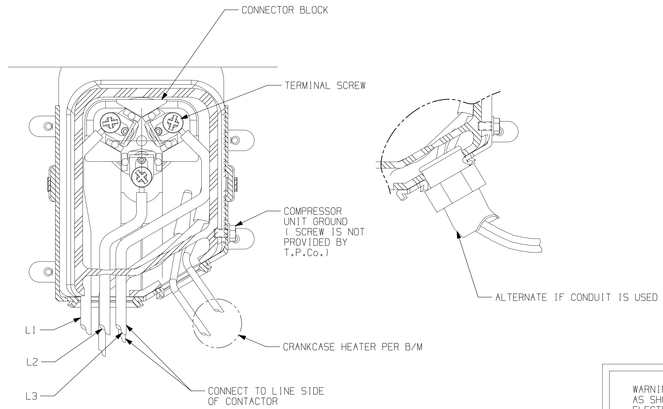
SCHEMATIC WIRING DIAGRAM - 3 PHASE INTERNAL OVERLOAD (LINE BREAK) AND CRANKCASE HEATER.
