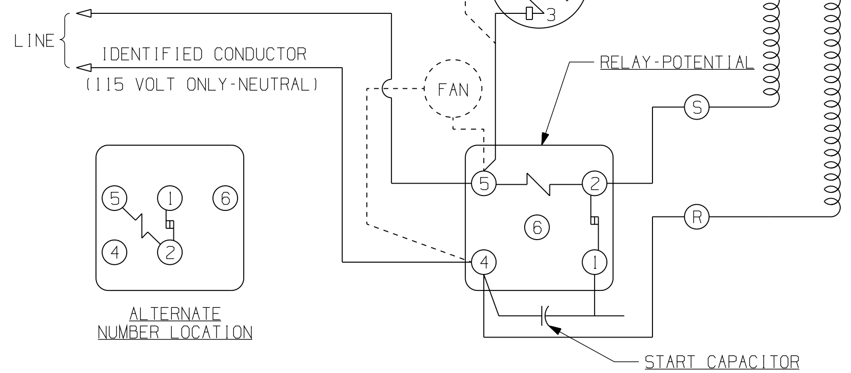
115 OR 230 V.-SCHEMATIC WIRING DIAGRAM - CSIR - POTENTIAL RELAY (REF. DWG. MD472-10)
