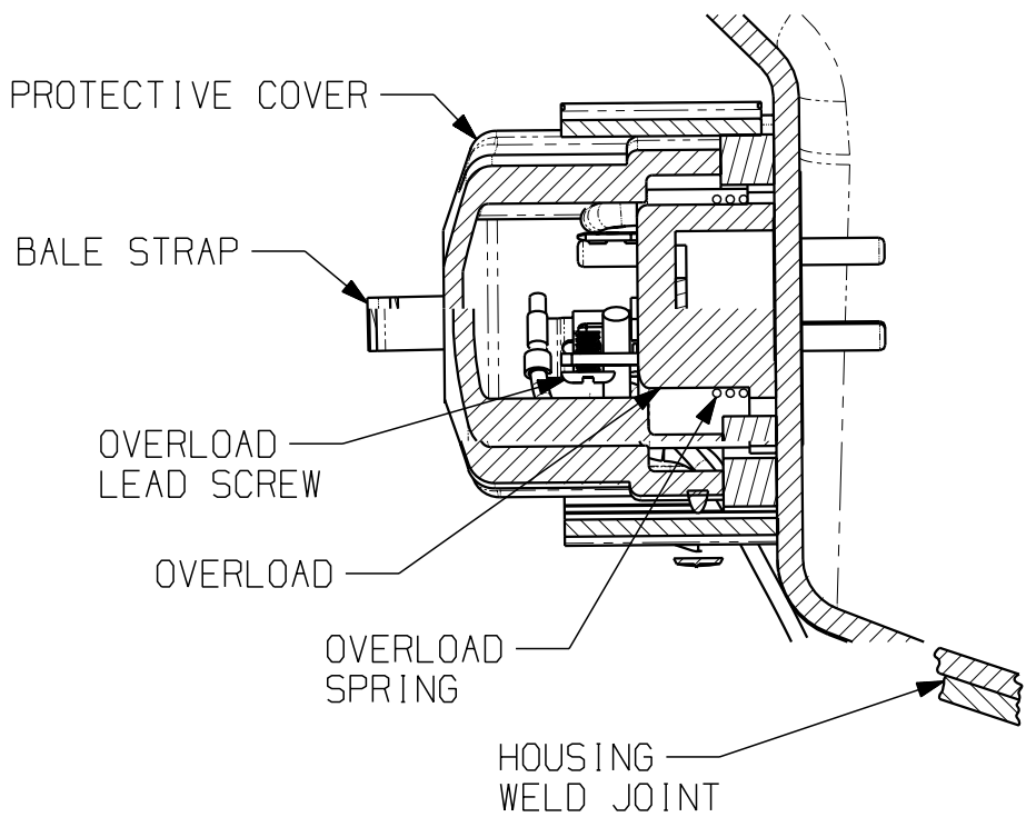
SECTION C-C
