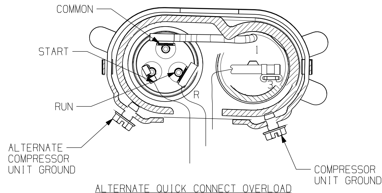
ALTERNATE B-B
