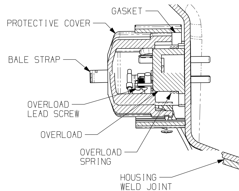
SECTION C-C
