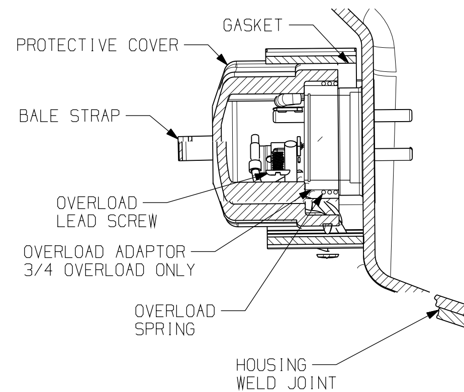
ALTERNATE C-C
