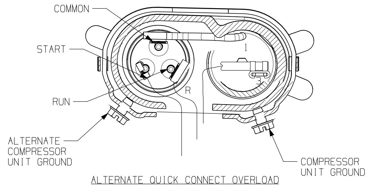
ALTERNATE B-B
