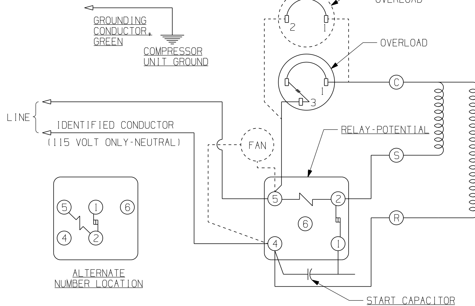
115 OR 230 V.-SCHEMATIC WIRING DIAGRAM - CSIR - POTENTIAL RELAY (REF. DWG. MD472-10)
