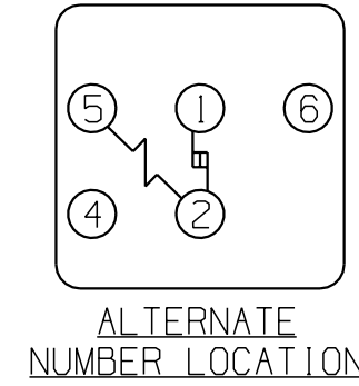
115 OR 230 V.-SCHEMATIC WIRING DIAGRAM - CSR OR CSR START CAPACITOR ASSIST (REF. DWG. MD472-35)
