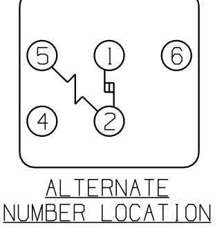
115 OR 230 V.-SCHEMATIC WIRING DIAGRAM - CSR OR CSR START CAPACITOR ASSIST (REF. DWG. MD472-35)
