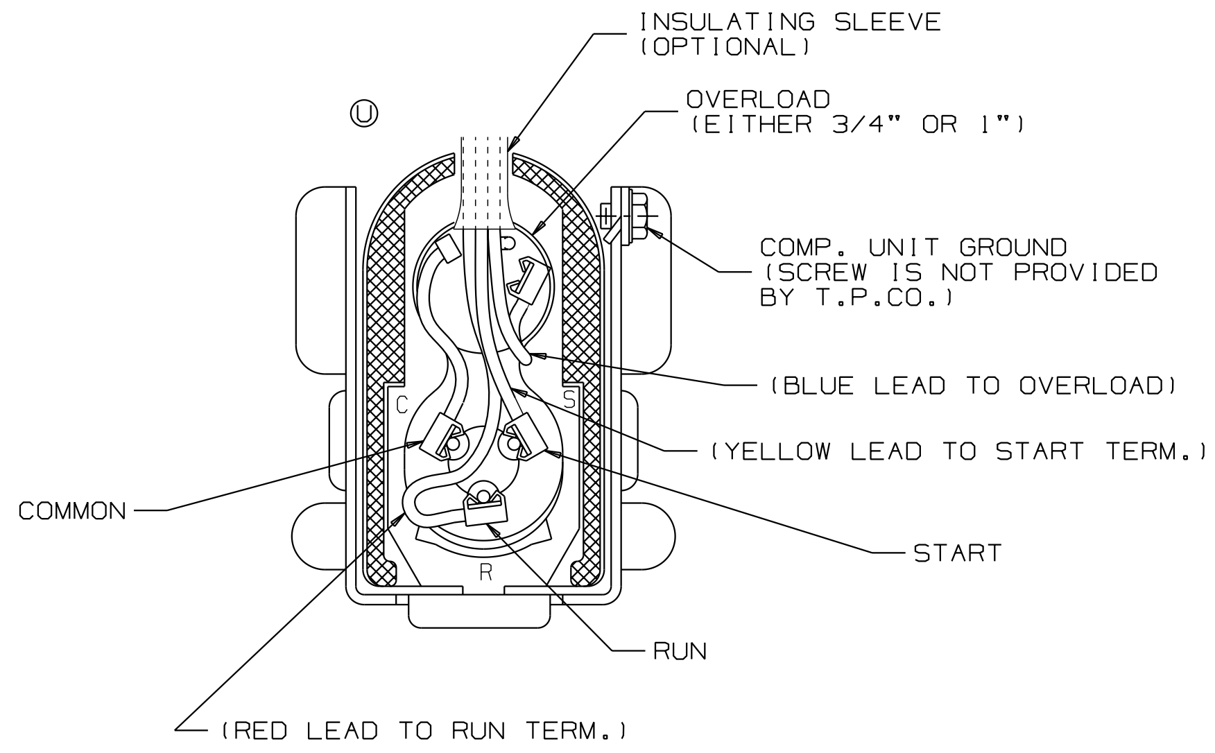
ELECTRICAL HOOK-UP REF. DEAK1
