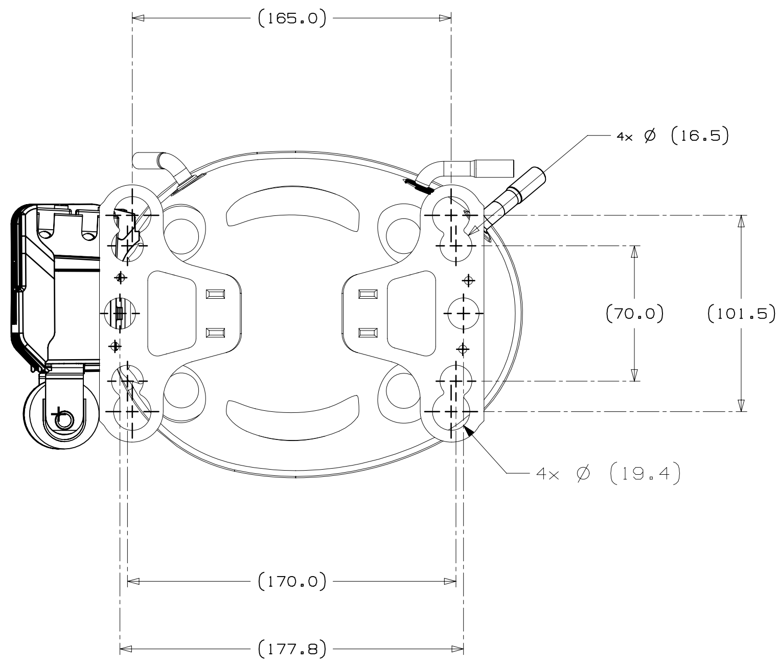
AUXILIARY VIEW FIXING DIMENSIONS
