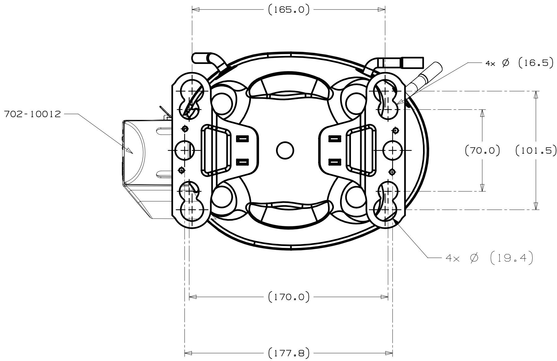
AUXILIARY VIEW FIXING DIMENSIONS
