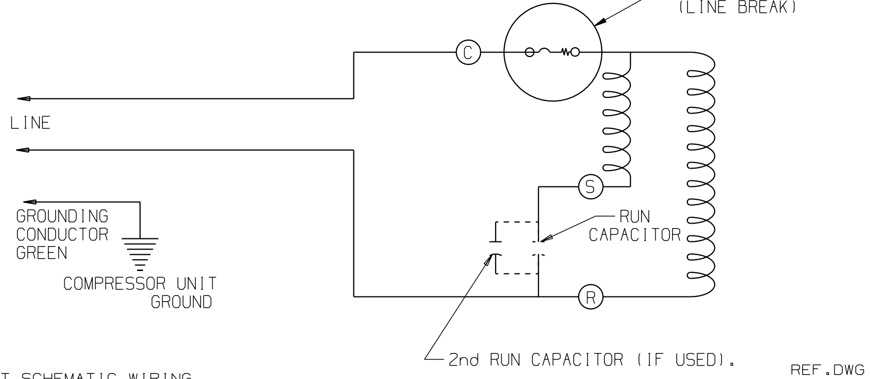
230 VOLT SCHEMATIC WIRING DIAGRAM-PSC-INTERNAL OVERLOAD (LINE BREAK)
