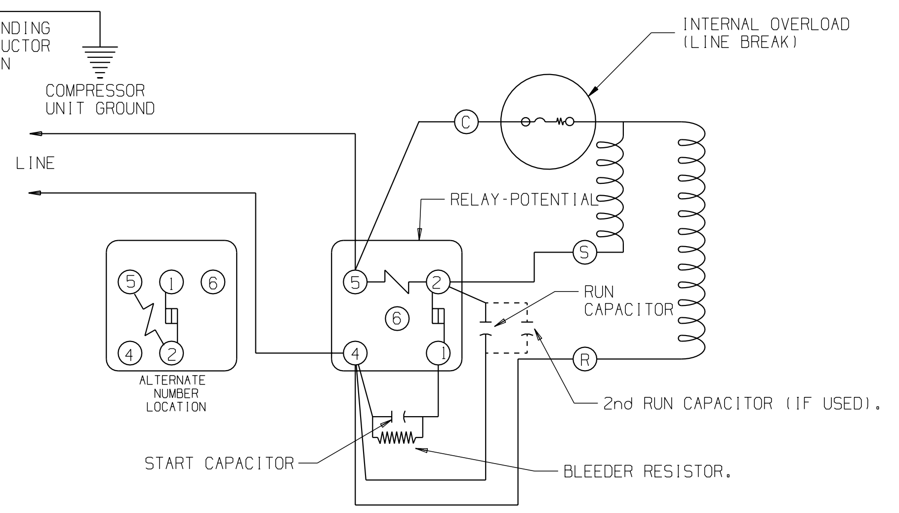
230 VOLT SCHEMATIC WIRING DIAGRAM-CSR OR CSR START CAPACITOR ASSIST -INTERNAL OVERLOAD (LINE BREAK)-REF.DWG.MD472-69
