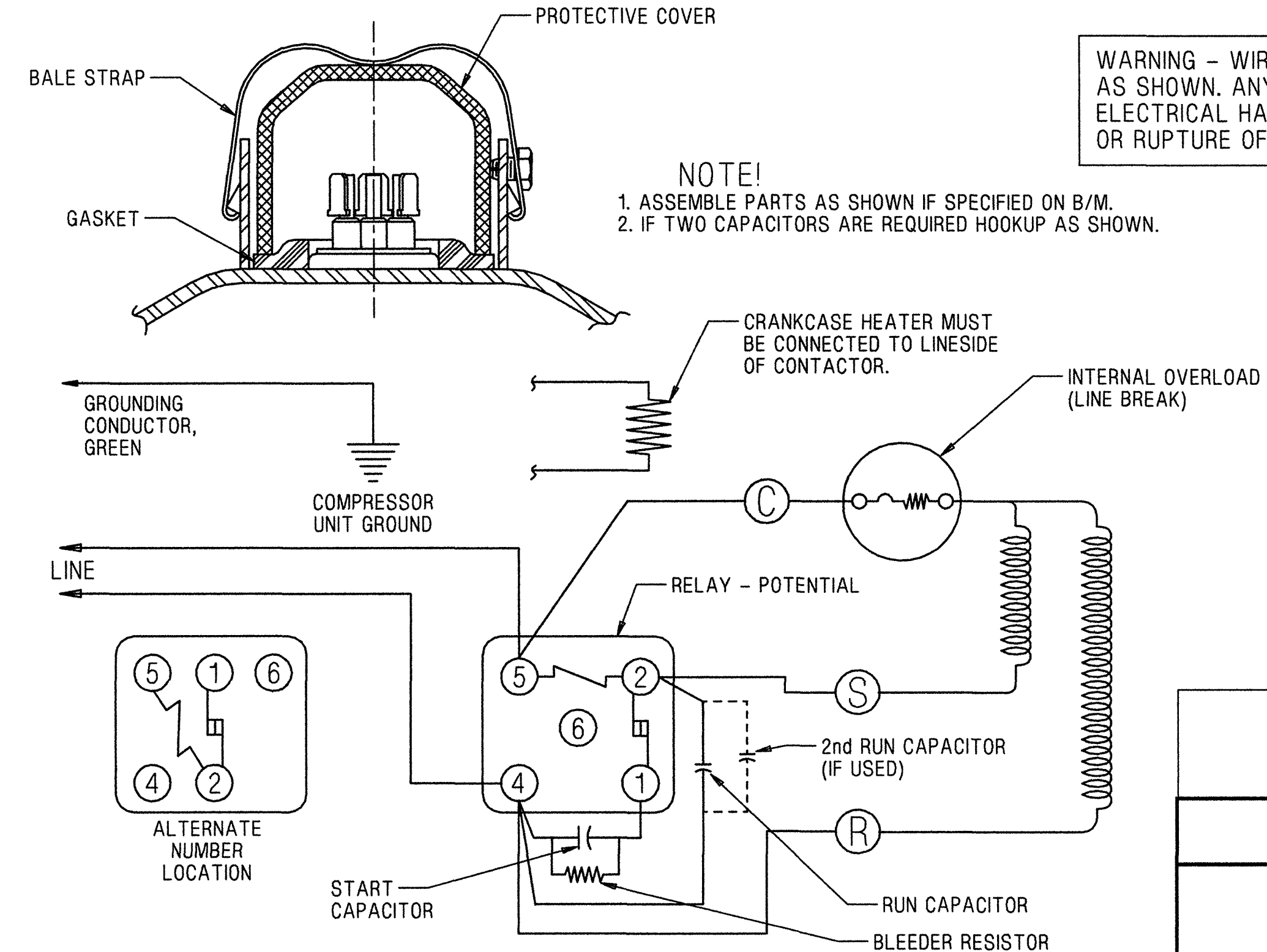
230 VOLT - SCHEMATIC WIRING DIAGRAM - CSR OR CSR START CAPACITOR ASSIST INTERNAL OVERLOAD (LINE BREAK) - CRANKCASE HEATER REF. DWG. MD472-66
