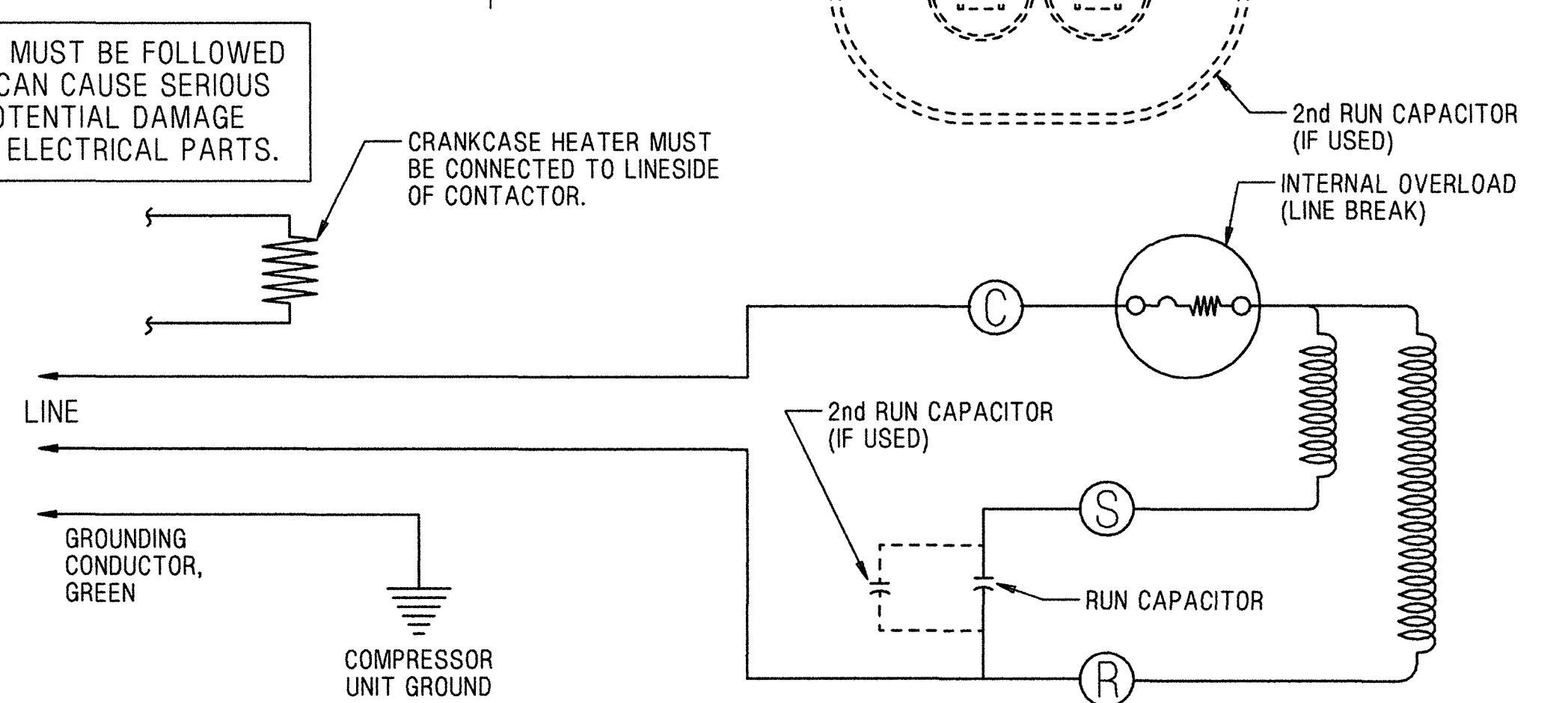
230 VOLT - SCHEMATIC WIRING DIAGRAM - PSC - INTERNAL OVERLOAD (LINE BREAK) - CRANKCASE HEATER.
