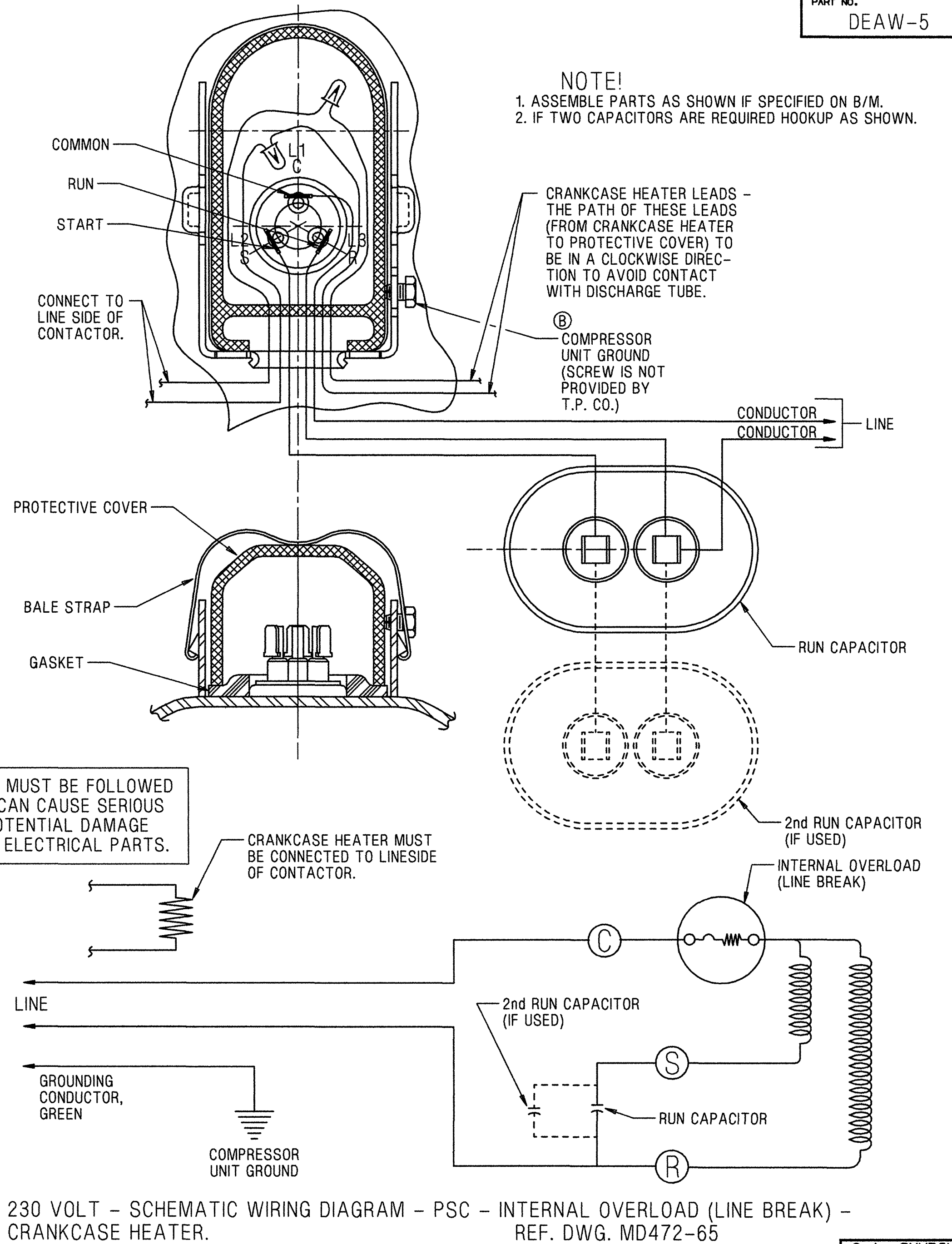
230 VOLT - SCHEMATIC WIRING DIAGRAM - PSC - INTERNAL OVERLOAD (LINE BREAK) - CRANKCASE HEATER.
