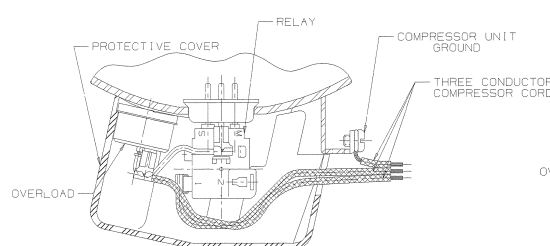
ALTERNATE RELAY (SCREW TYPE)
