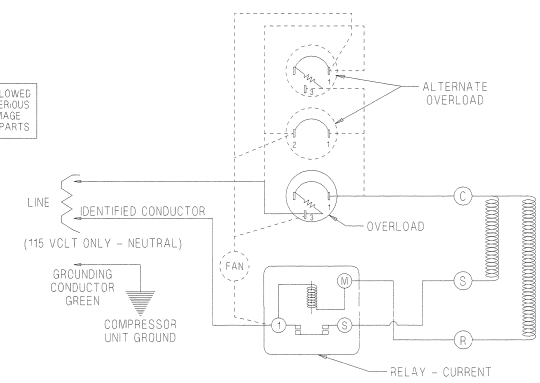
115 OR 230 VOLT - SCHEMATIC WIRING DIAGRAM - RSIR REF. DWG. MD-472
