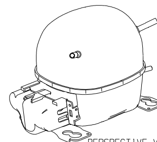
PERSPECTIVE VIEW SCALE 1:4
