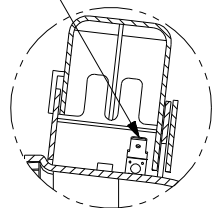
PARTIAL SECTION F-F SCALE: 1:1 (INTERNAL TO BOX) (NON PAINTED AREA)
