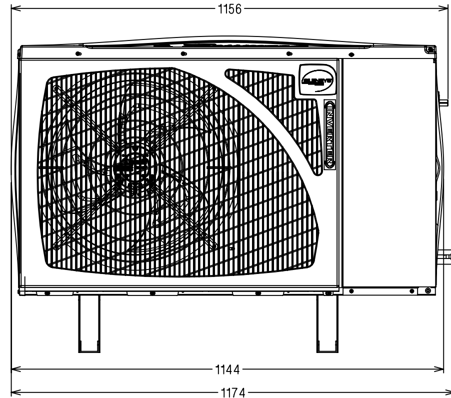
Grille de ventilation Railing of ventilation
