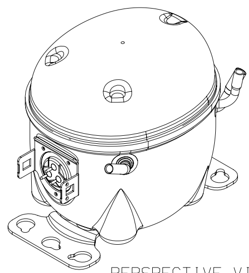
PERSPECTIVE VIEW SCALE 1:3
