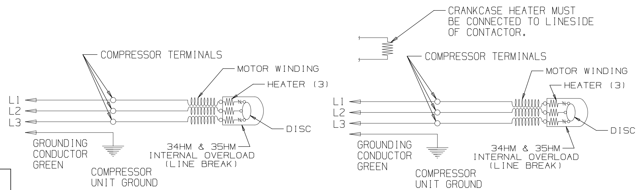
SCHEMATIC WIRING DIAGRAM - 3 PHASE INTERNAL OVERLOAD (LINE BREAK) REF DWG MD472-24
