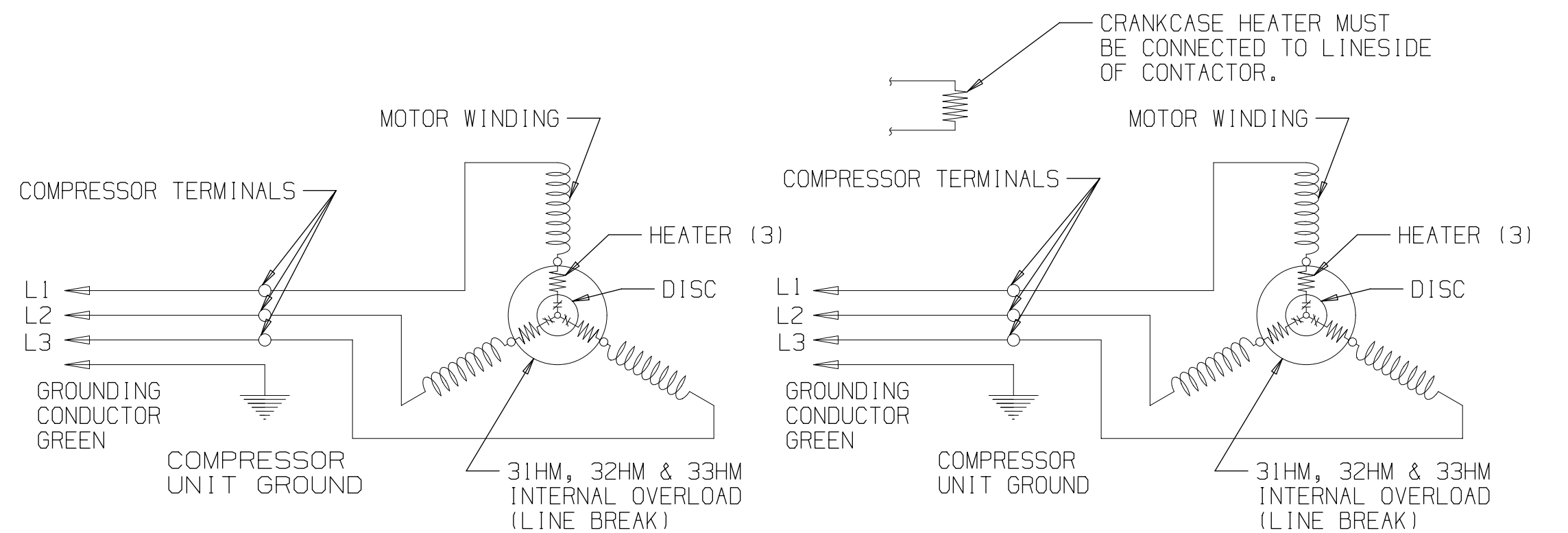
SCHEMATIC WIRING DIAGRAM - 3 PHASE INTERNAL OVERLOAD (LINE BREAK) REF DWG MD472-24
