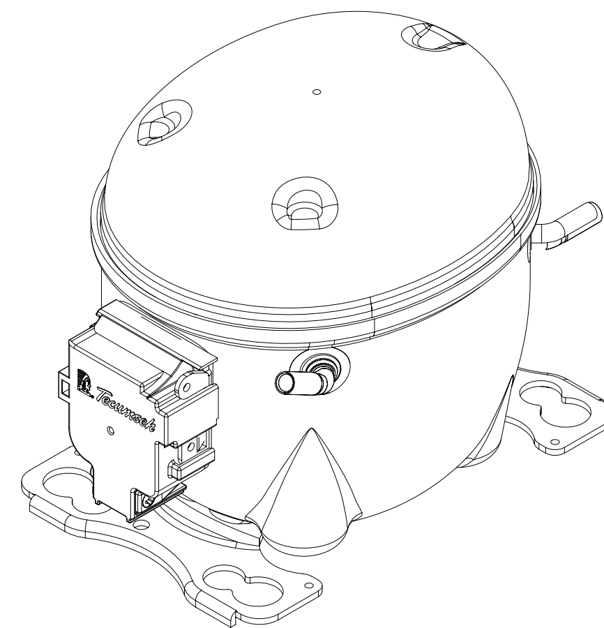
PERSPECTIVE VIEW SCALE 1:2
